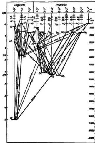
The atomic state of Cadmium
