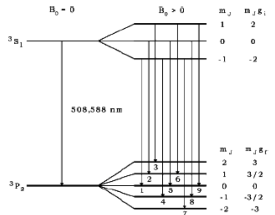
Energy shift of the atomic states
