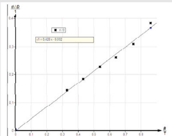
Measurement of results for \delta/\Delta against magnetic field strength
