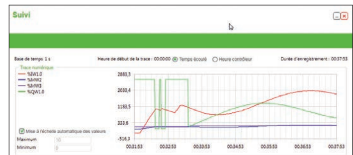
Visualization of the setpoint and PID output curves
