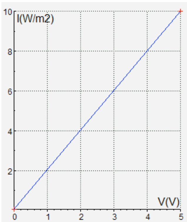
Figure 2. Calibration graph (range 0 .. 10 \text{W/m}^2 ) of the Light sensor in the standard sensor library in the Coach program.
