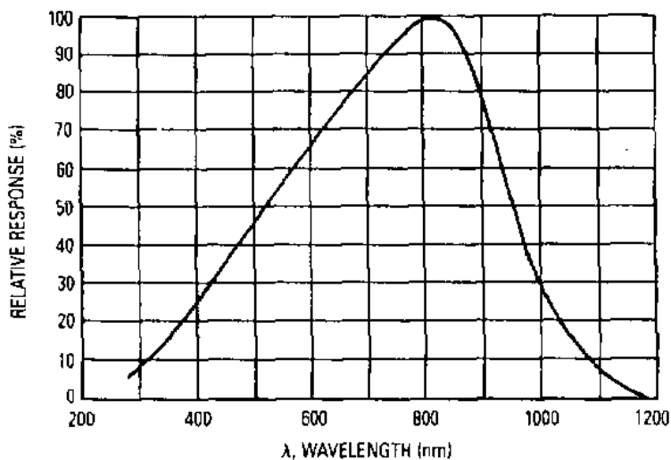
Figure 3. Relative spectral response of the Light sensor
